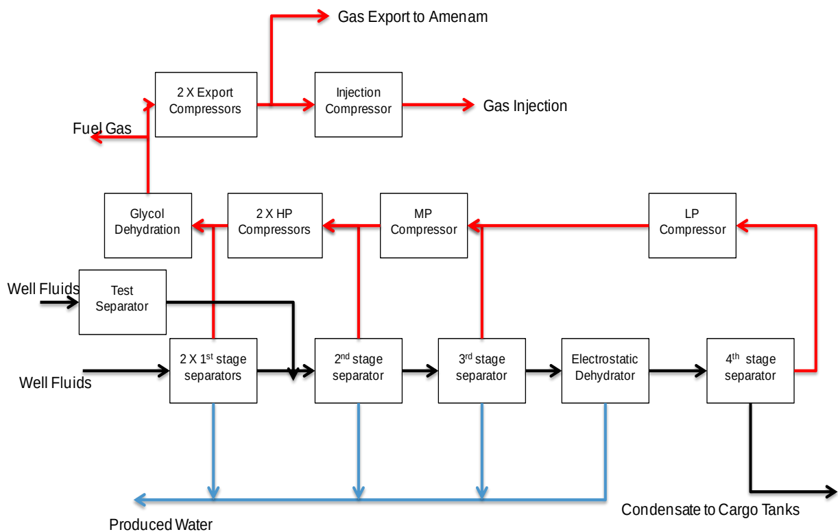
Figure 16-12 Akpo Process Flow Diagram
