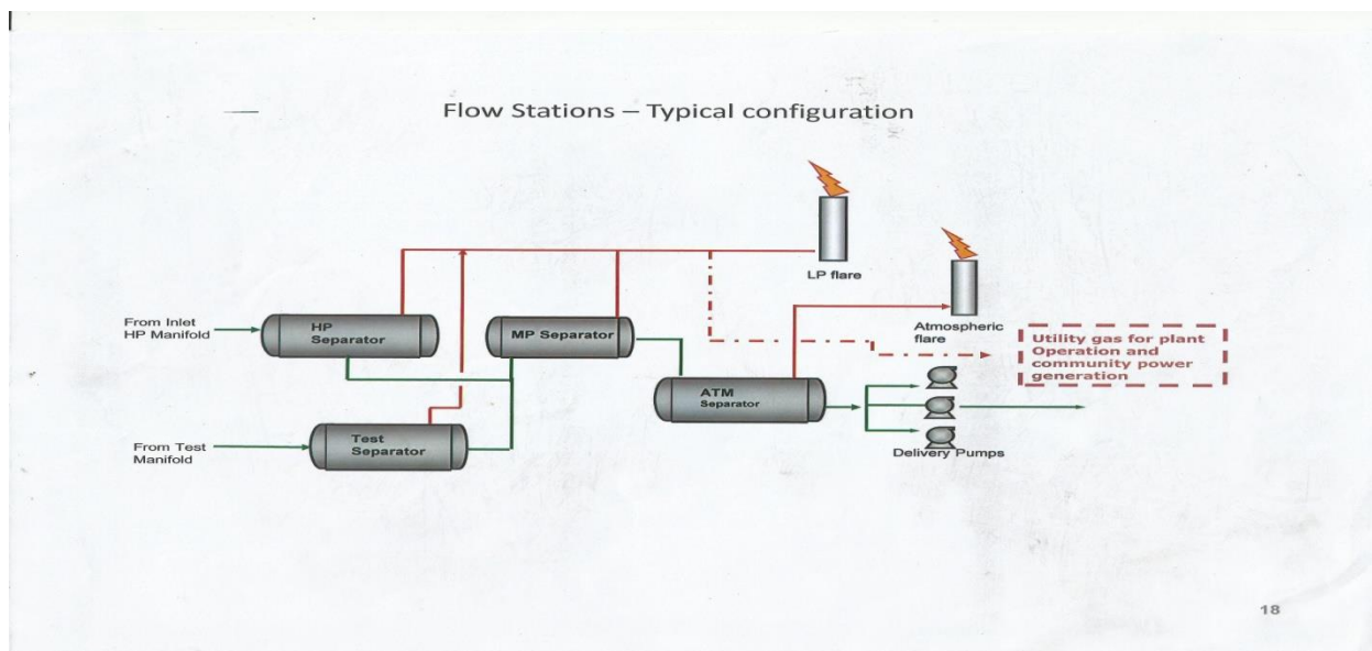
Figure 16-4 Flow Station Configuration
