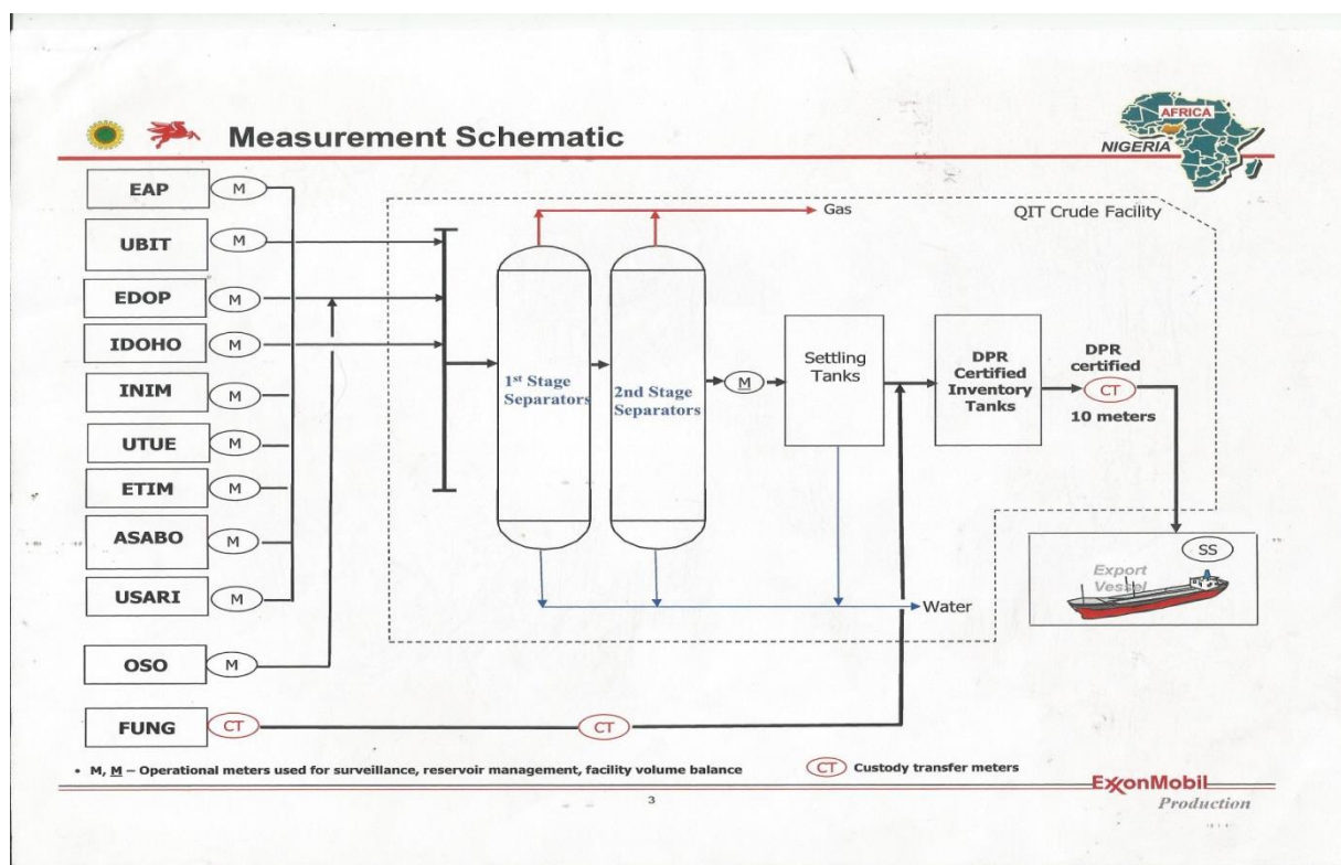
Figure 16-5 Measurement Schematics
