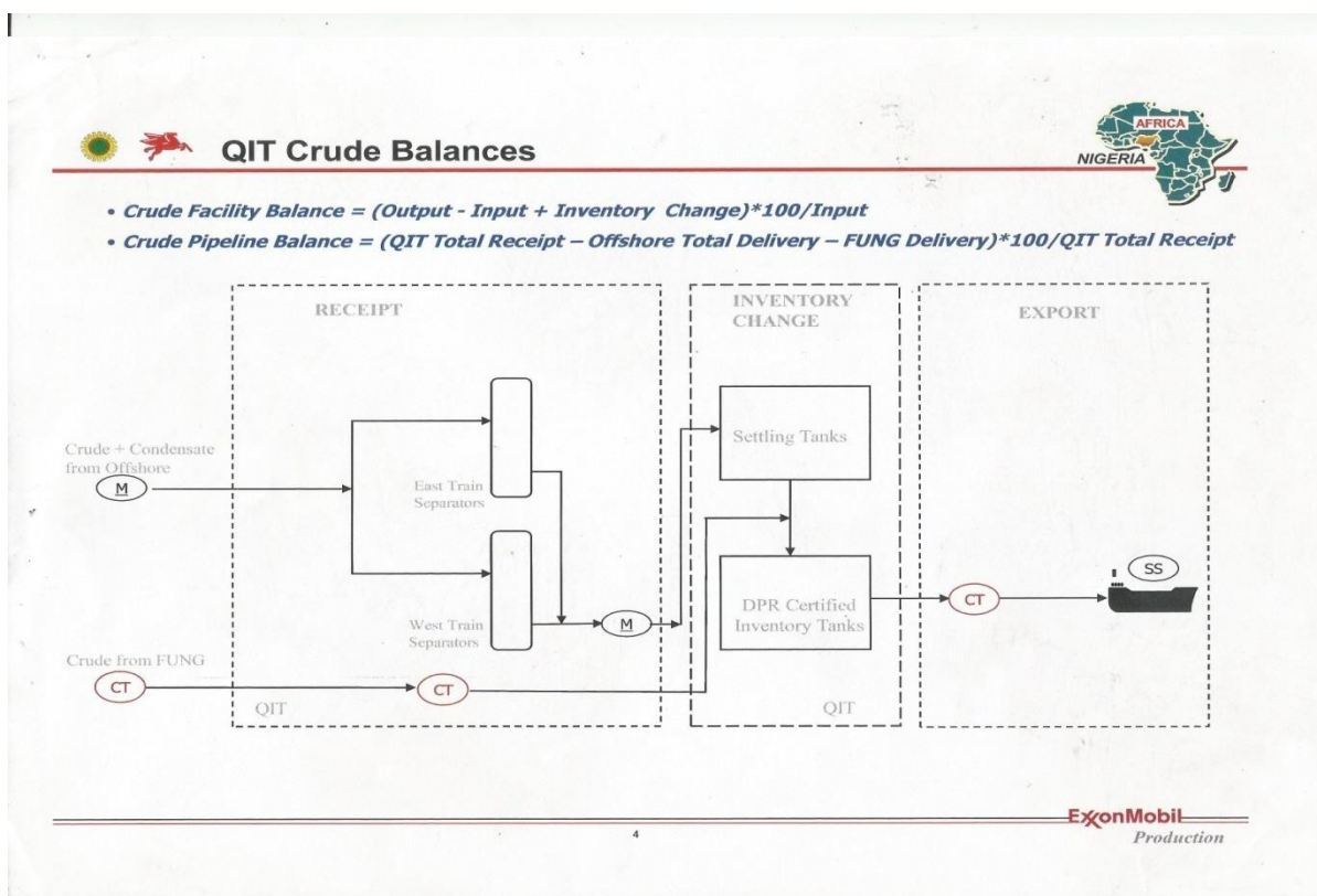
Figure 16-6 QIT Crude Oil Balances
