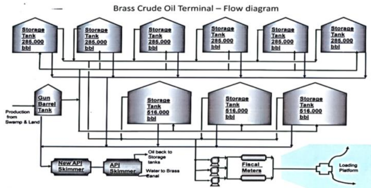
Figure 16-1 Brass Crude Oil Terminal – Flow diagram
