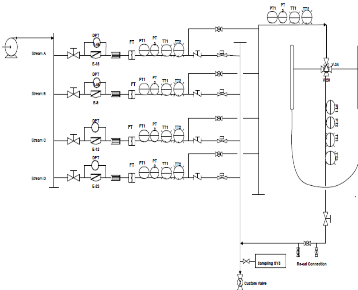
Figure 16-13 FSO Oil Custody Transfer Metering Above
