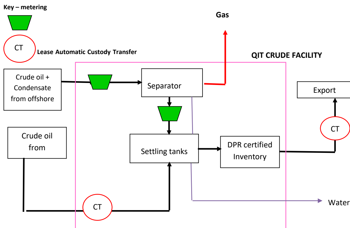
Figure 16-7 Process Schematic Metering System
